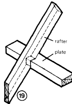
Birdsmouth
