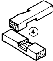
Dovetailed cross-halving
