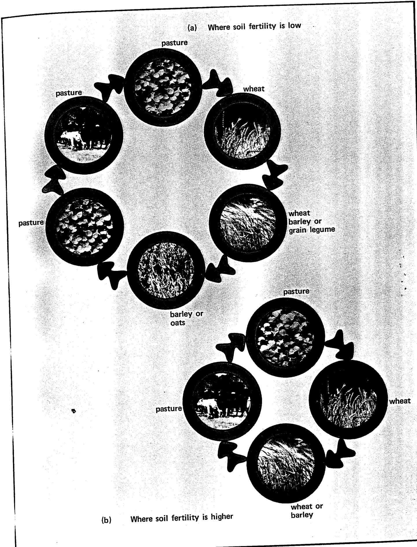
Fig. 10 Typical rotations using subterranean clover (a) where soil fertility is low, and (b) where soil fertility is higher.
