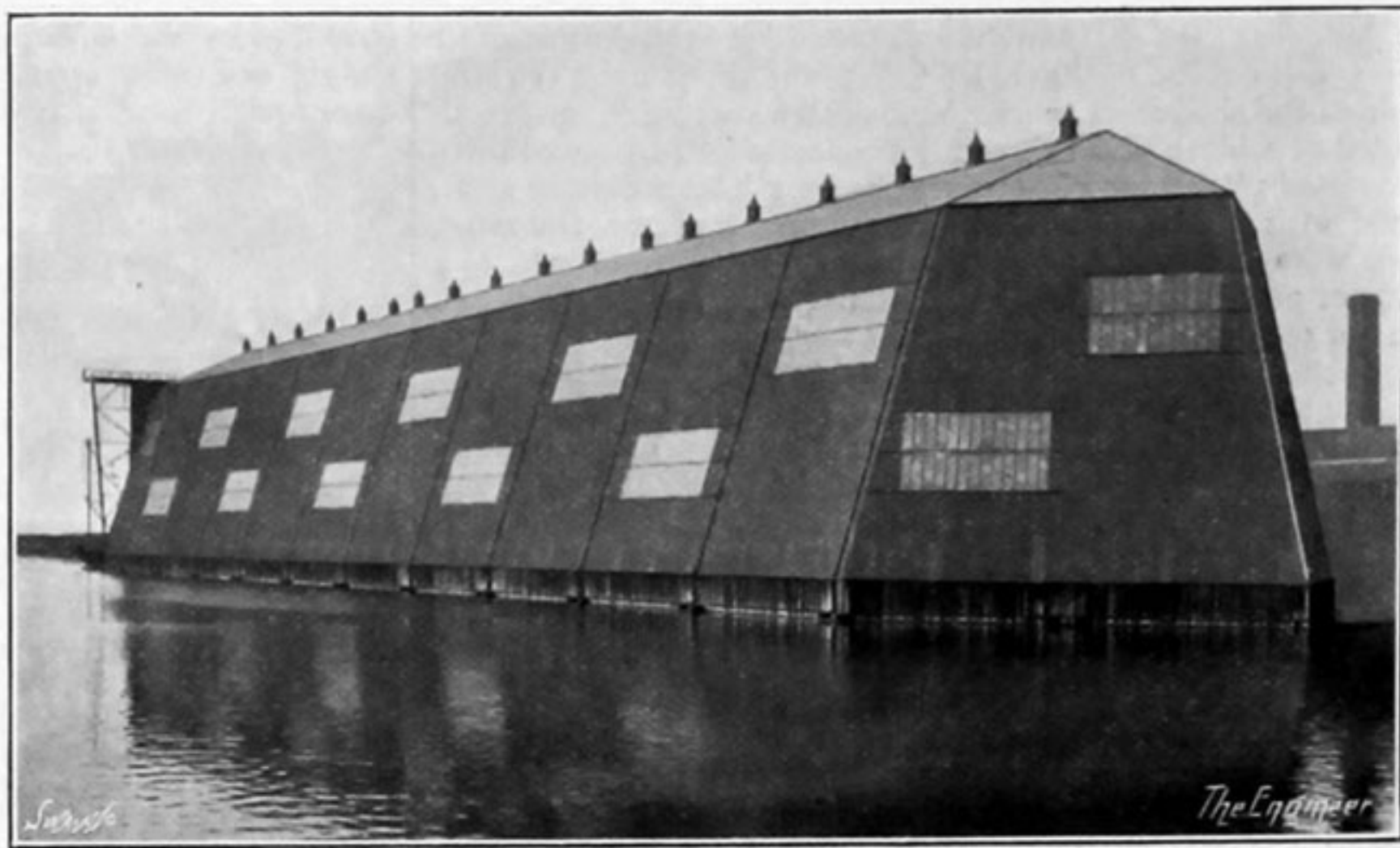
Fig. 2—COMPLETE SHED, VEE-SHAPED END
