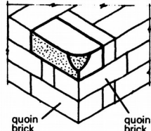
② Single bull nose stop
