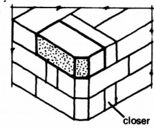
③ Cant brick
