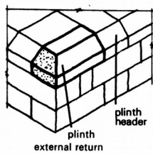
⑤ Plinth brick (splay)
